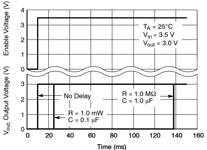
Figure 21. Delayed Turn-on
